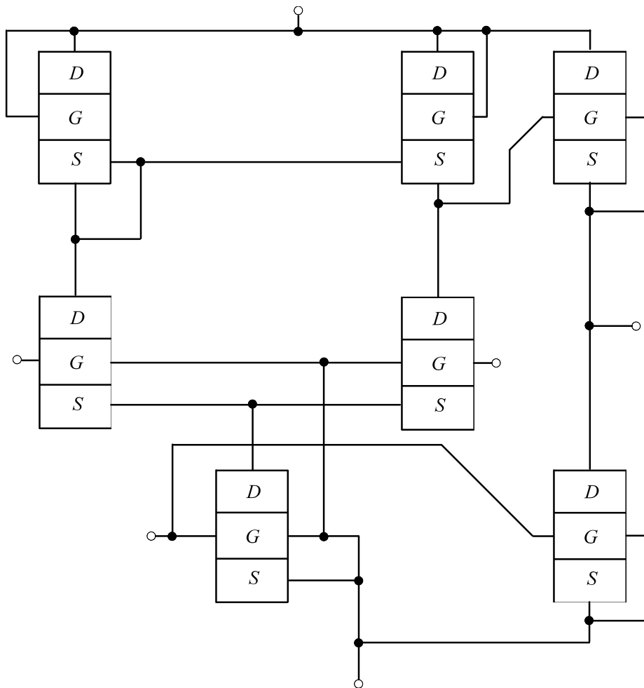
Figure 1a: Structure of the considered comparator [19]
