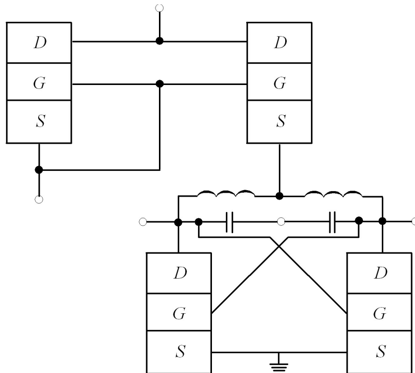
Figure 1: The considered injection locked oscillator [4]
