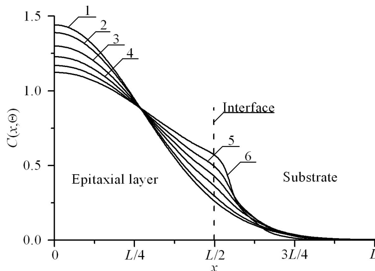
Figure 2a: Dependences of concentration of dopant, infused in heterostructure from Figs. 1, on coordinate in direction, which is perpendicular to interface between epitaxial layer substrate. Difference between values of dopant diffusion coefficient in layers of heterostructure increases with increasing of number of curves. Value of dopant diffusion coefficient in the epitaxial layer is larger, than value of dopant diffusion coefficient in the substrate
