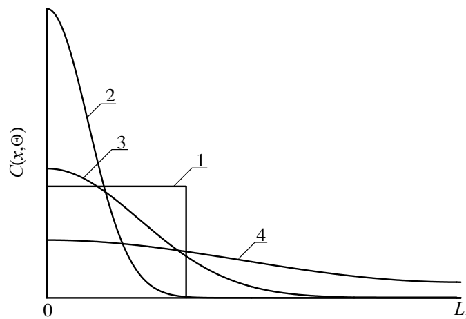
Figure 4a: Distributions of concentration of infused dopant in depth of heterostructure from Fig. 1 for different values of annealing time (curves 2-4) and idealized step-wise approximation (curve 1). Increasing of number of curve corresponds to increasing of annealing time
