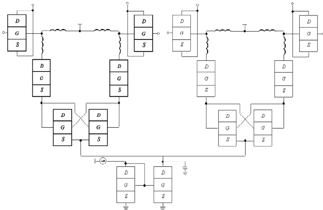
Figure 1: The considered oscillator [4]
