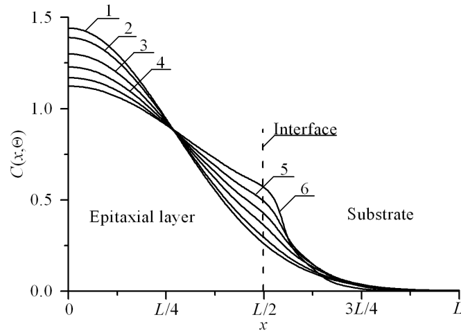
Figure 2a: L Dependences of concentration of dopant, infused in heterostructure from Figs. 1, on coordinate in direction, which is perpendicular to interface between epitaxial layer substrate. Difference between values of dopant diffusion coefficient in layers of heterostructure increases with increasing of number of curves. Value of dopant diffusion coefficient in the epitaxial layer is larger, than value of dopant diffusion coefficient in the substrate
