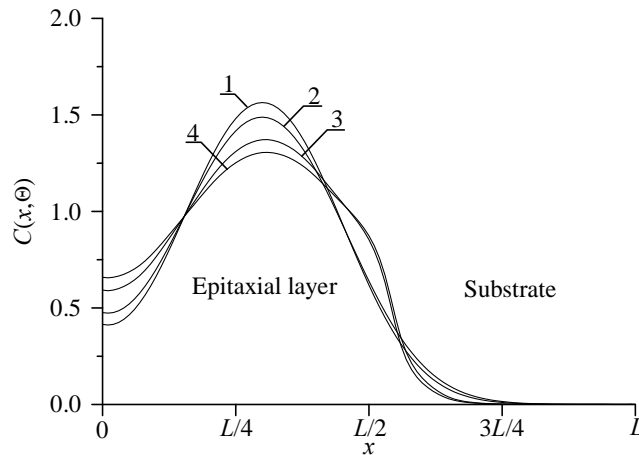
Figure 2b: Dependences of concentration of dopant, implanted in heterostructure from Figs. 1, on coordinate in direction, which is perpendicular to interface between epitaxial layer substrate. Difference between values of dopant diffusion coefficient in layers of heterostructure increases with increasing of number of curves. Value of dopant diffusion coefficient in the epitaxial layer is larger, than value of dopant diffusion coefficient in the substrate. Curve 1 corresponds to homogenous sample and annealing time \Theta = 0.0048 (L_x^2 + L_y^2 + L_z^2)/D_0 . Curve 2 corresponds to homogenous sample and annealing time \Theta = 0.0057 (L_x^2 + L_y^2 + L_z^2)/D_0 . Curves 3 and 4 correspond to heterostructure from Figs. 1; annealing times \Theta = 0.0048 (L_x^2 + L_y^2 + L_z^2)/D_0 and \Theta = 0.0057 (L_x^2 + L_y^2 + L_z^2)/D_0 , respectively
