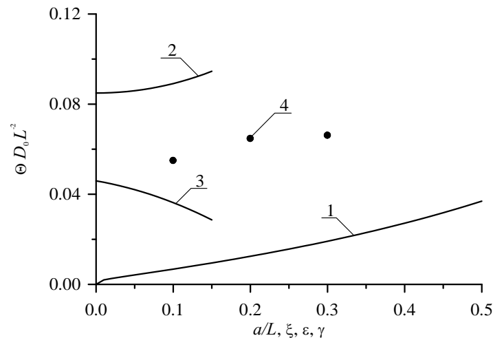
Figure 5b: Dimensionless optimal annealing time of implanted dopant as a function of several parameters. Curve 1 describes the dependence of the annealing time on the relation a/L and \xi = \gamma = 0 for equal to each other values of dopant diffusion coefficient in all parts of heterostructure. Curve 2 describes the dependence of the annealing time on value of parameter e for a/L=1/2 and \xi = \gamma = 0 . Curve 3 describes the dependence of the annealing time on value of parameter \xi for a/L=1/2 and \epsilon = \gamma = 0 . Curve 4 describes the dependence of the annealing time on value of parameter \gamma for a/L=1/2 and \epsilon = \xi = 0
