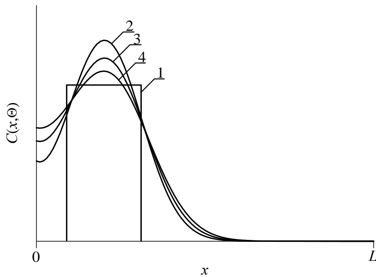
Figure 4b: Distributions of concentration of implanted dopant in depth of heterostructure from Fig. 1 for different values of annealing time (curves 2-4) and idealized step-wise approximation (curve 1). Increasing of number of curve corresponds to increasing of annealing time
