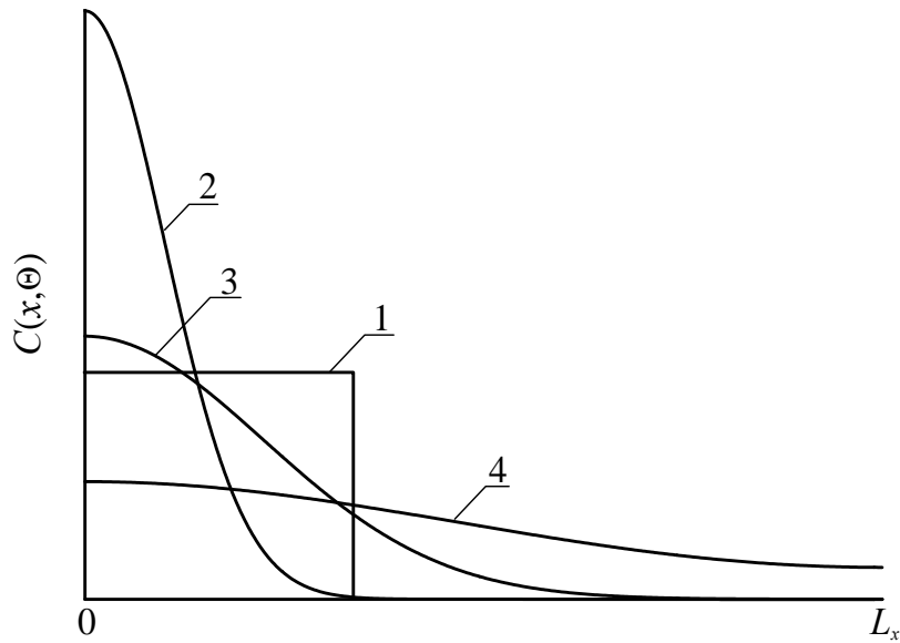
Figure 4a: Distributions of concentration of infused dopant in depth of heterostructure from Fig. 1 for different values of annealing time (curves 2-4) and idealized step-wise approximation (curve 1). Increasing of number of curve corresponds to increasing of annealing time
