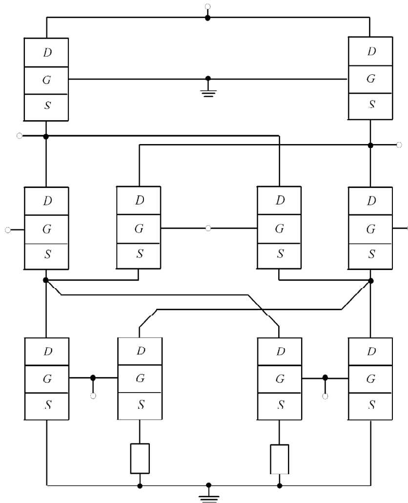
Figure 1a: Structure of the considered mixer [19]
