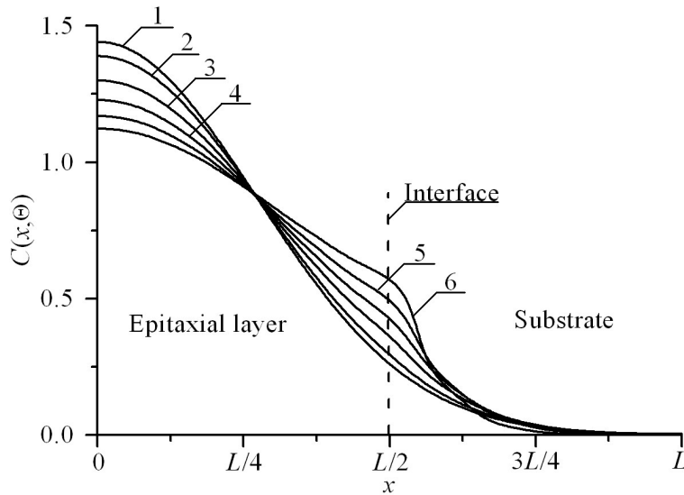
Figure 2: Distributions of concentration of infused dopant in heterostructure from Fig. 1 in direction, which is perpendicular to interface between epitaxial layer substrate. Increasing of number of curve corresponds to increasing of difference between values of dopant diffusion coefficient in layers of heterostructure under condition, when value of dopant diffusion coefficient in epitaxial layer is larger, than value of dopant diffusion coefficient in substrate
